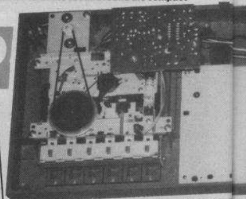
Laid bare, with its works there for all to see: the Spectrum Plus 2, a tidied up version of the 128. On the far left is the underside of the Datacorder, while heatsinks abound round the compact circuit board.
